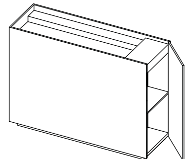
FSC33 w1200 x d400 x h900mm bowl width 976mm
