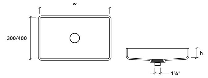
w1000mm x d300mm
