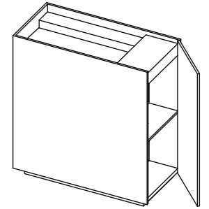
FSC31 w840 x d400 x h900mm bowl width 616mm
