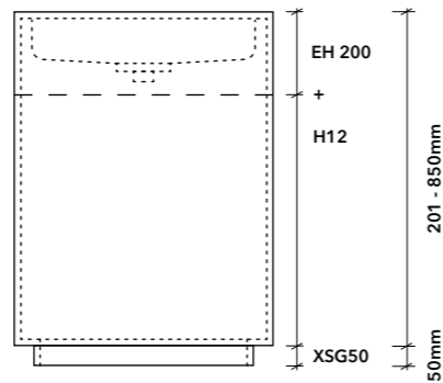
EH200 + remaining m 2 in H12 Edge 201 - 850mm high
