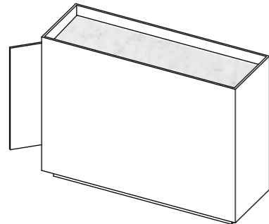
FSC53 w1200 x d400 x h900mm bowl width 1176mm
