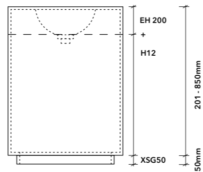
EH200 + remaining m² in H12 Edge 201 - 850mm high
