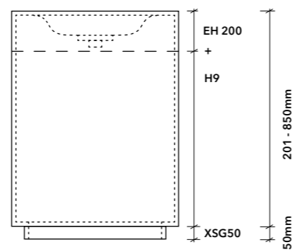
EH200 + remaining m 2 in H9 Edge 201 - 850mm high
