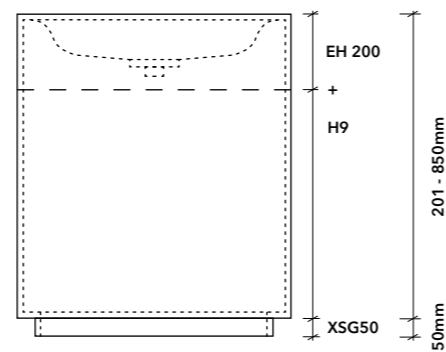
EH200 + remaining m 2 in H9 Edge 201 - 850mm high
